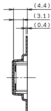
SECT. E-E
