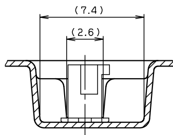
SECT. F-F
