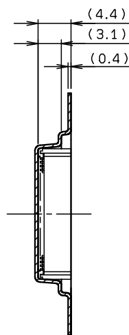
SECT. E-E
