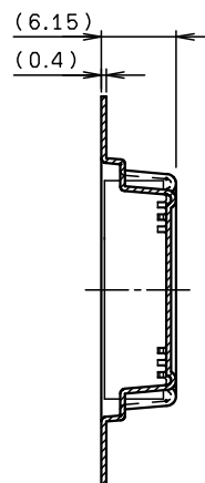
SECT. F-F (11~31P)
