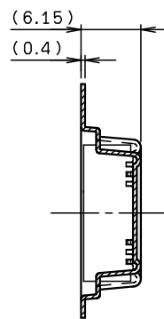
SECT. F-F (3~10P)
