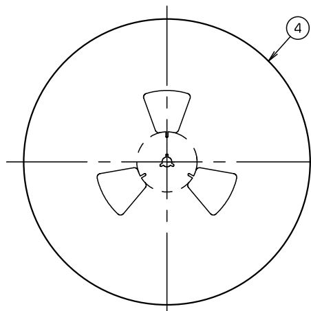
REEL DIMENSION (S=1:5) (3~31P)
