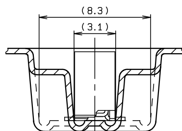
SECT. D-D (S=5:1)
