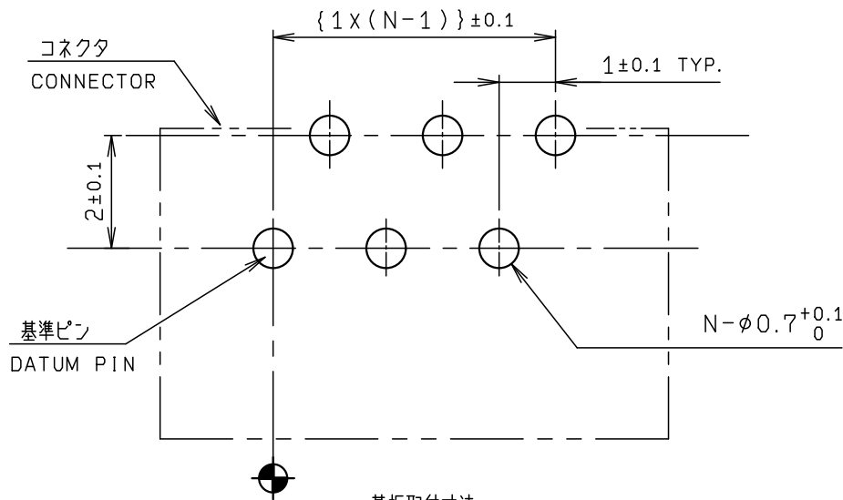
基板取付寸法 MOUNTING LAYOUT (t=1.2~1.6)
