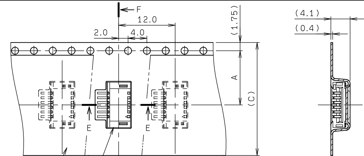
SECT. F-F (3~10P)
