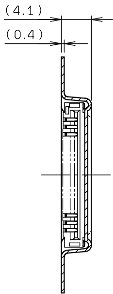
SECT. F-F (3~10P)
