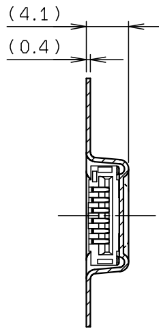
SECT. F-F (3~10P)
