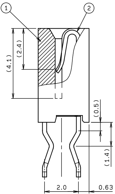
SECT. X-X (S=10/1)
