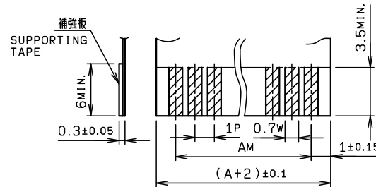
SECT. X-X (S=10/1)
