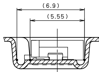
SECT. E-E (S=6:1)
