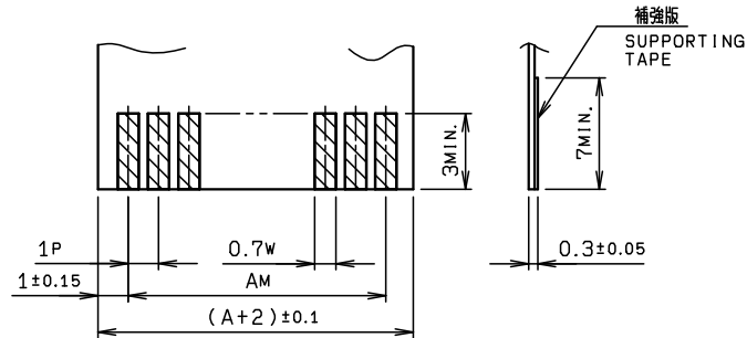
適用FPC/FFC寸法 APPLICABLE FPC/FFC
