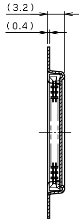
SECT. F-F (12~20P)
