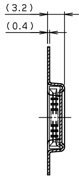
SECT. F-F (5~11P)
