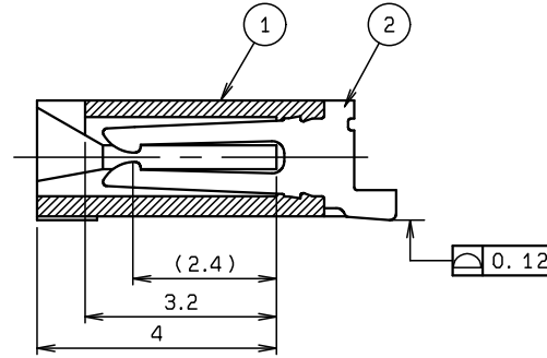
SECT. X-X (S=10:1)
