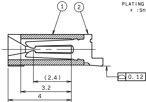
SECT. X-X (S=10/1)
