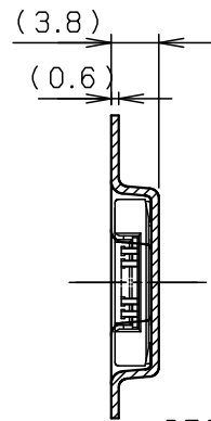
SECT. D-D (5~11P)
