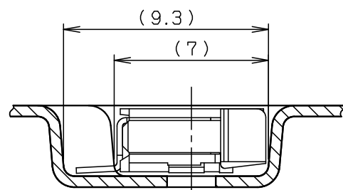
SECT. E-E (S=4:1)
