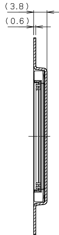
SECT. D-D (12~30P)
