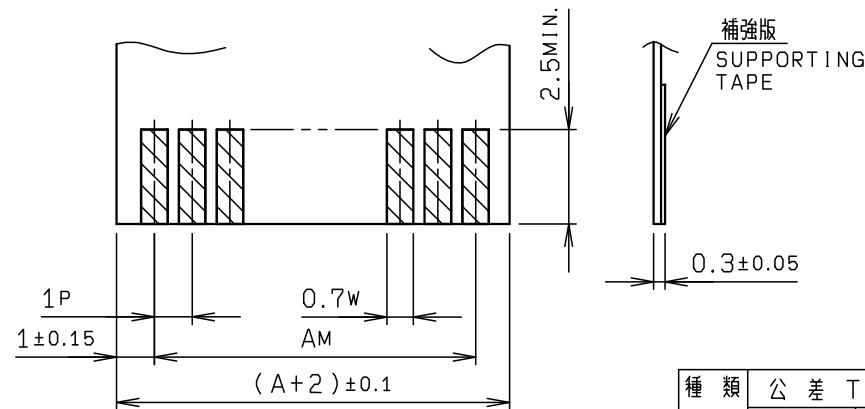
適用AuめっきFPC APPLICABLE Au PLATING FPC
