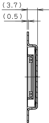
SECT. F-F (12~30P)
