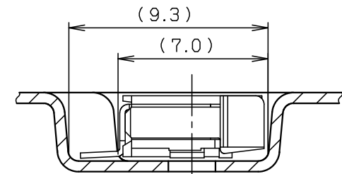
SECT. E-E (S=4:1)
