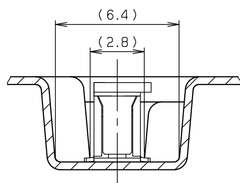
SECT. F-F (S=5:1)
