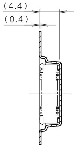
SECT. E-E (6~24P)
