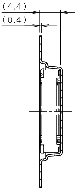
SECT. E-E (25~30P)
