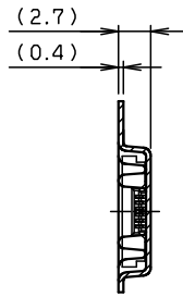
SECT. K-K
