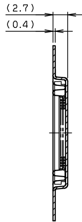
SECT. K-K (25~30P)
