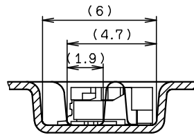
SECT. L-L (S=5:1)
