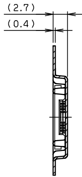
SECT. K-K (7~24P)
