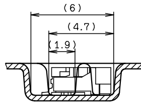
SECT. L-L (S=5:1)
