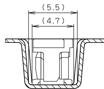
SECT. F-F (S=4:1)
