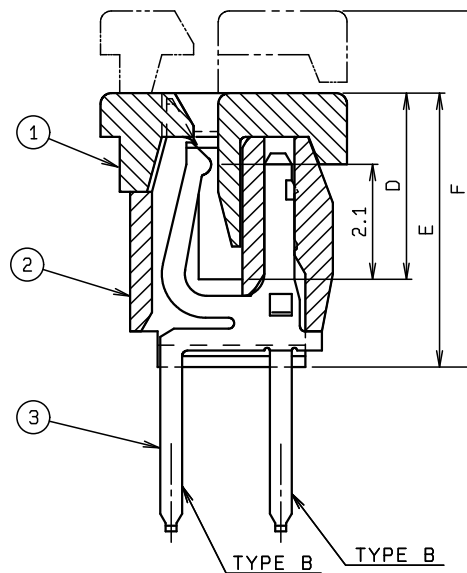
SECT. W-W (S=10:1)
