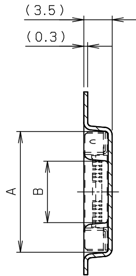
SECT. D-D
