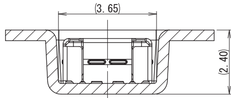
SECT. H-H (S=10:1)
