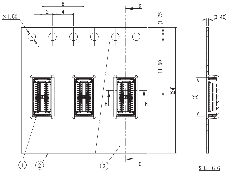
SECT. G-G
