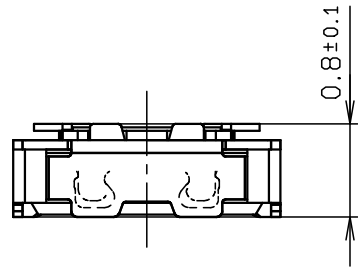
MATING CONDITION
