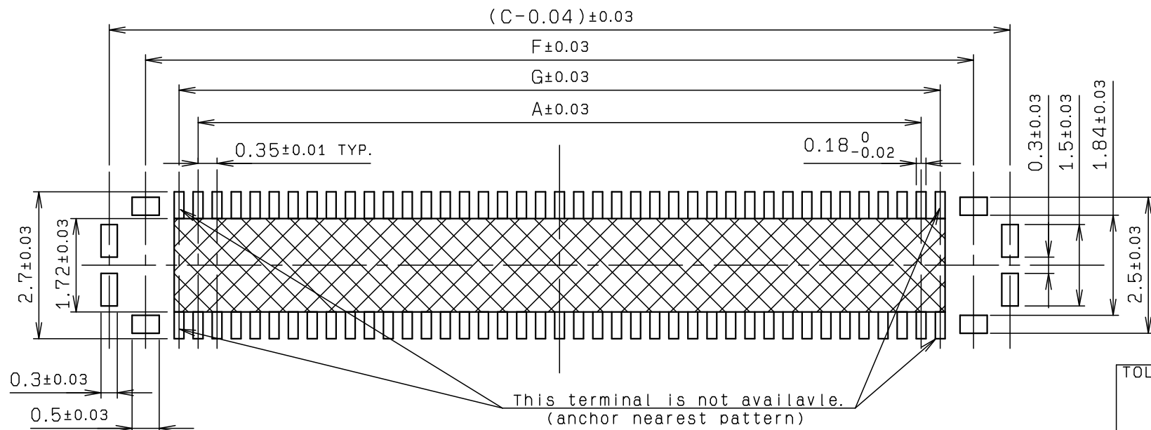
MOUNTING LAYOUT
