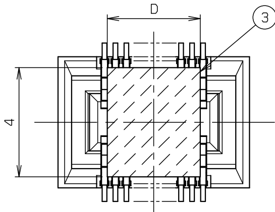
POSITION OF VACUUM TAPE
