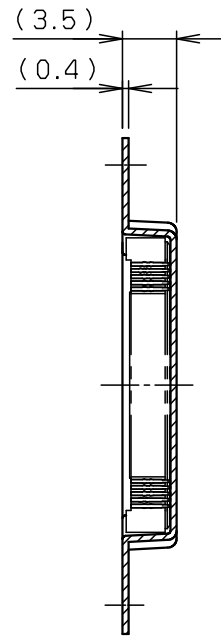
SECT. F-F
