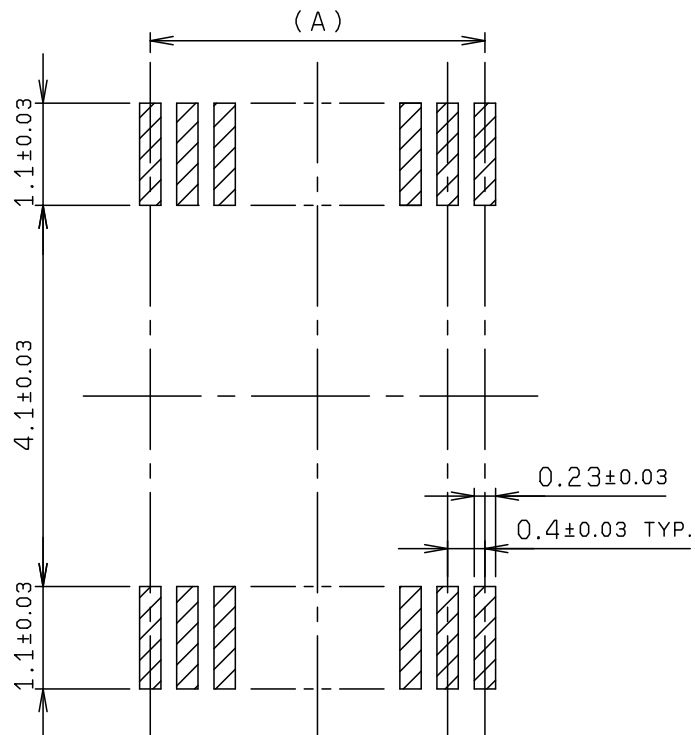
MOUNTING LAYOUT
