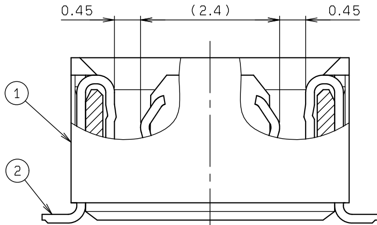
SECT. S-S
