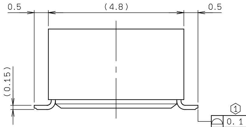
SECT. S-S
