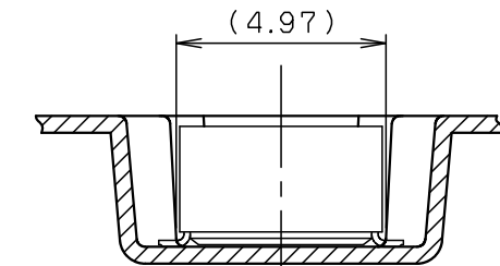
SECT. E-E
