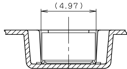
SECT. E-E
