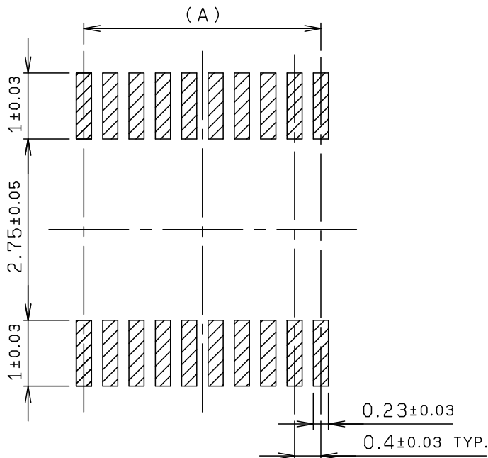
MOUNTING LAYOUT
