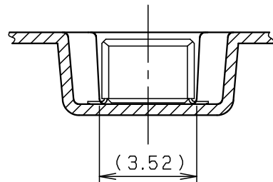
SECT. E-E
