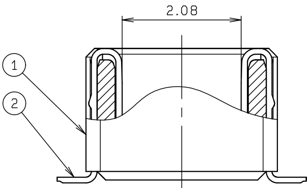
SECT. S-S
