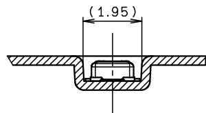
SECT. G-G (S=8:1)
