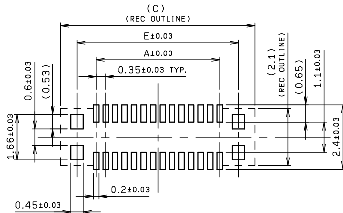
MOUNTING LAYOUT
