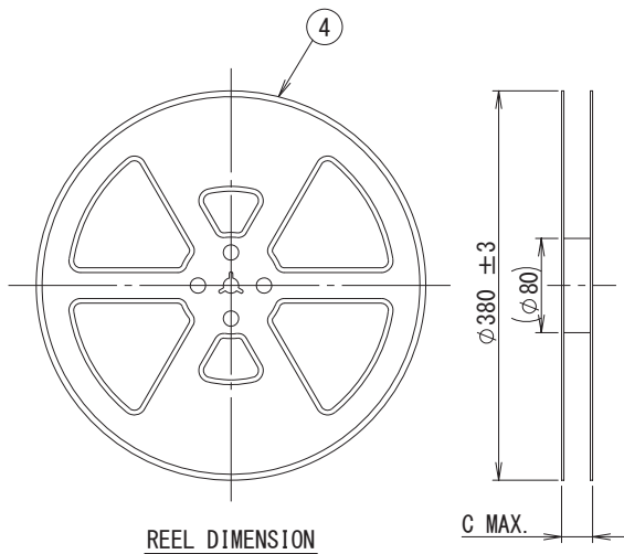
REEL DIMENSION
