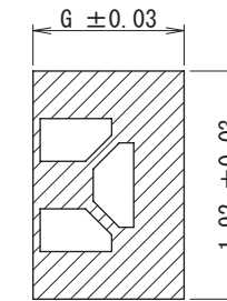
DETAIL "Y" ANCHOR PLATE PAD AREA
