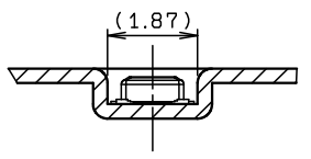
SECT. G-G (S=8:1)
