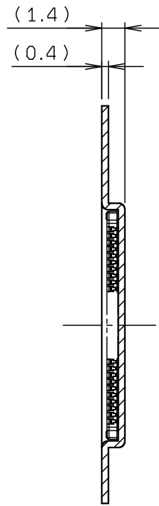
SECT. F-F
