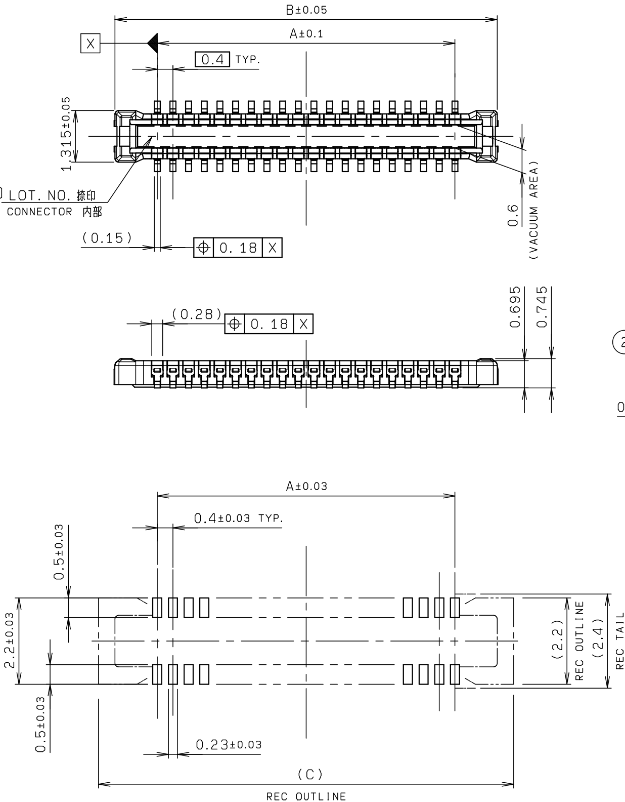
MOUNTING LAYOUT
