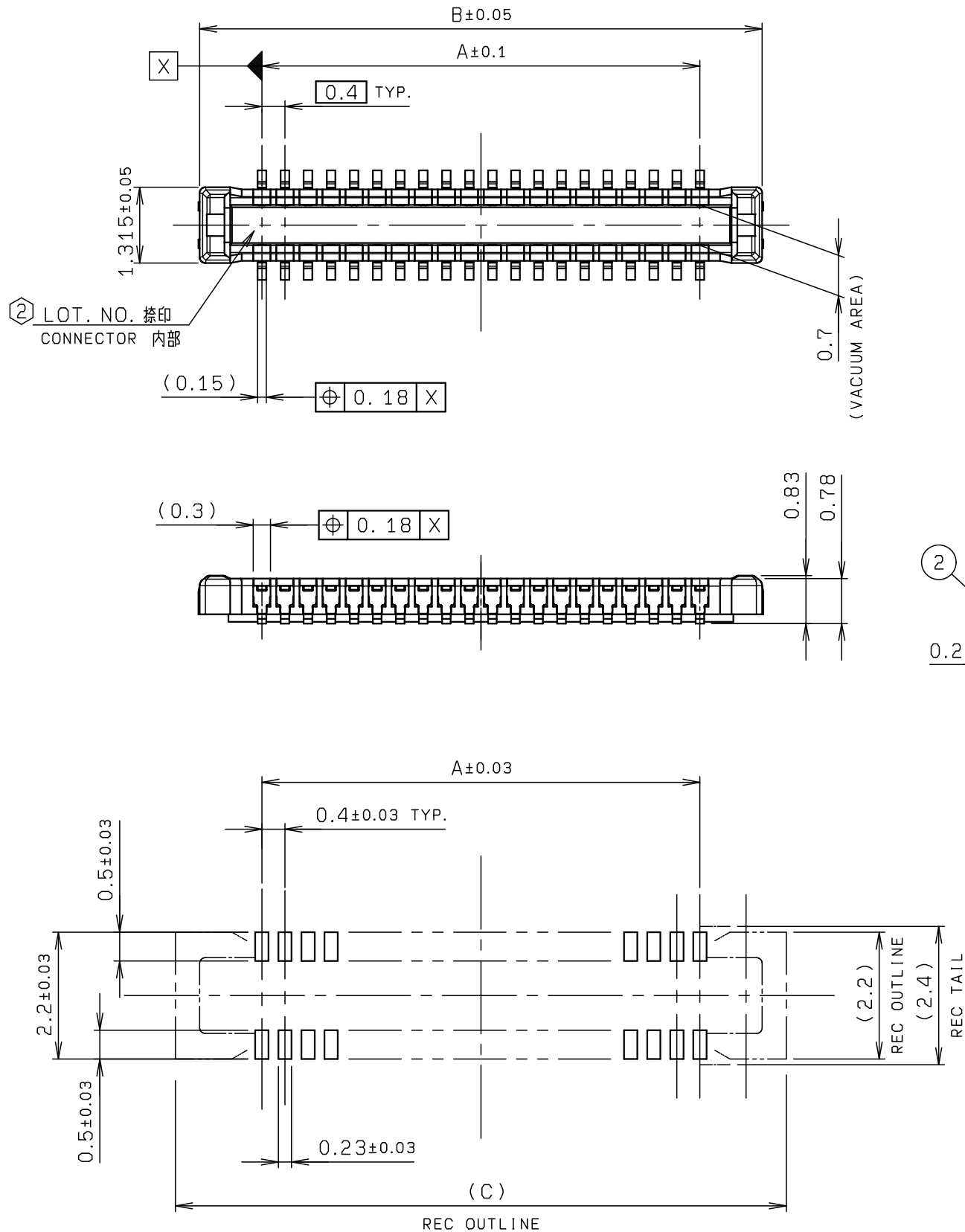
MOUNTING LAYOUT
