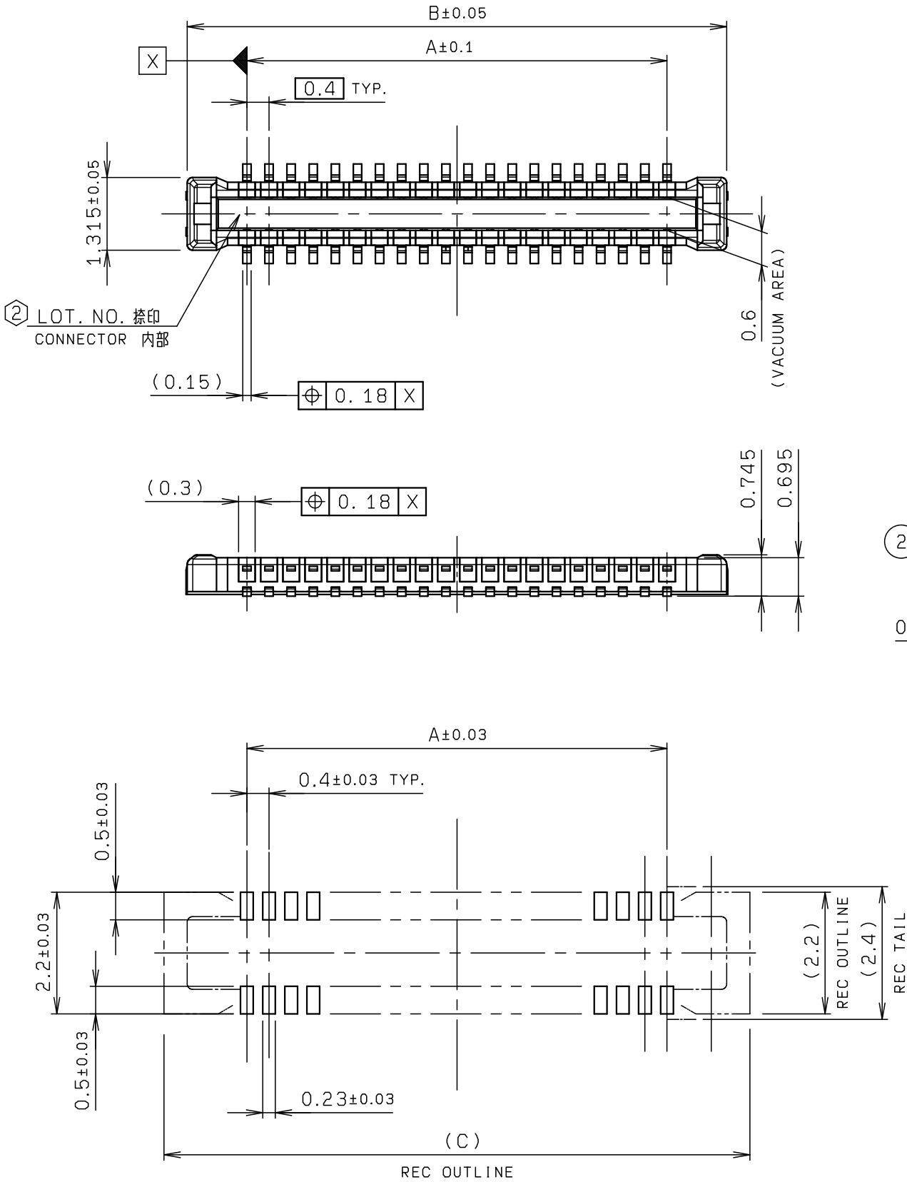
MOUNTING LAYOUT
