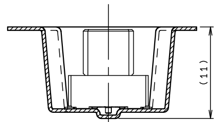
SECT. N-N
