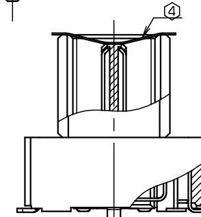
SECT. X-X
