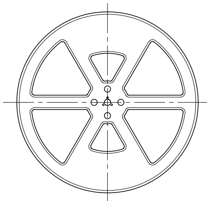
REEL DIMENSION (S=1:5)
