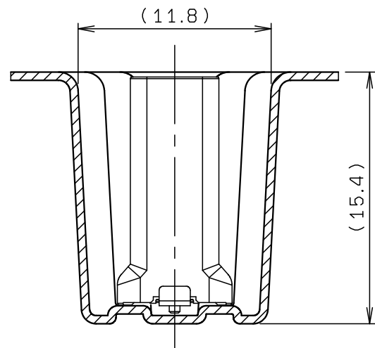
SECT. F-F (S=3:1)
