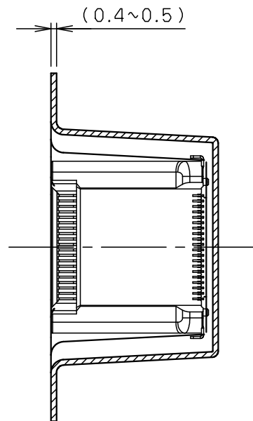
SECT. G-G
