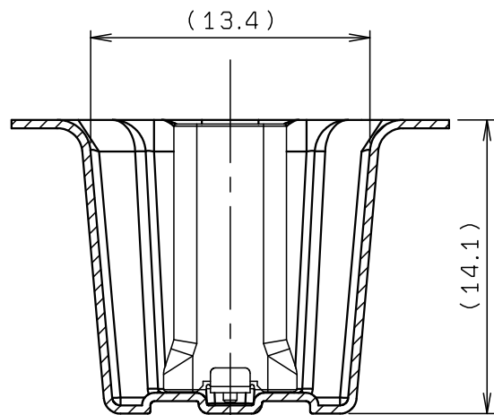
SECT. F-F (S=3:1)
