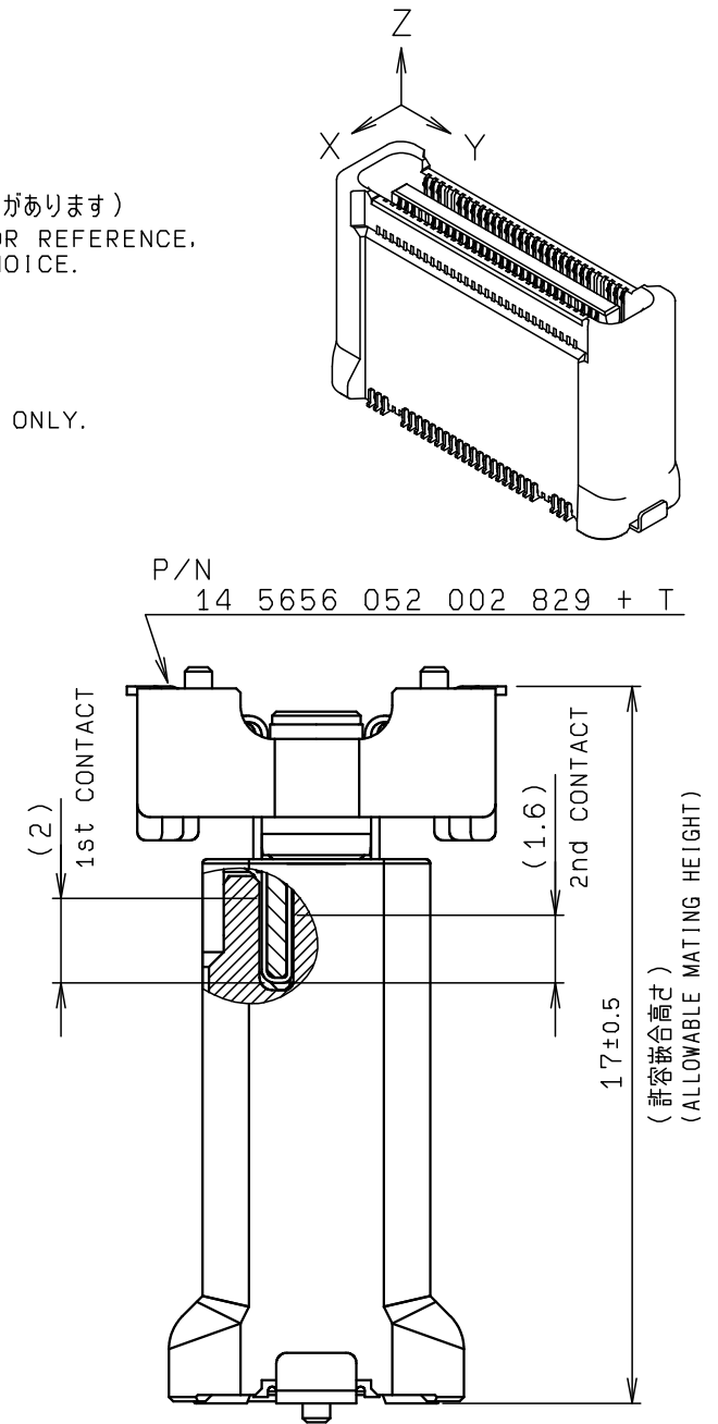
MATED CONDITION
