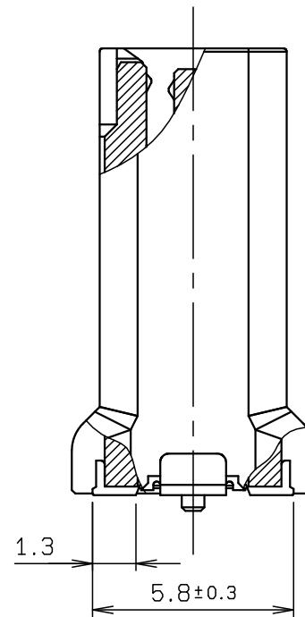
SECT. H-H
