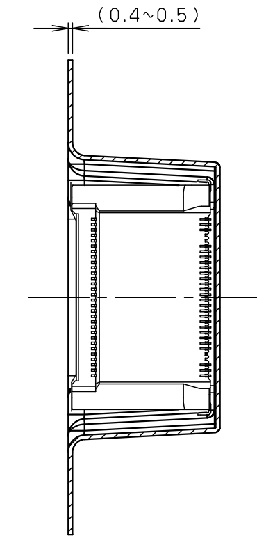
SECT. G-G
