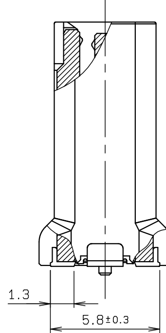
SECT. H-H
