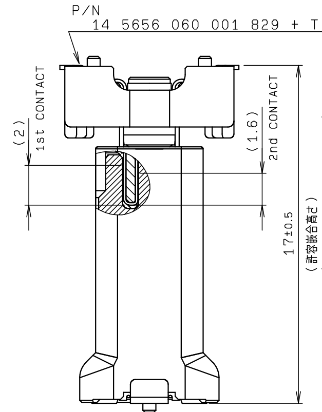
MATED CONDITION
