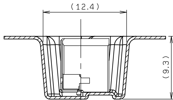
SECT. F-F (S=3:1)
