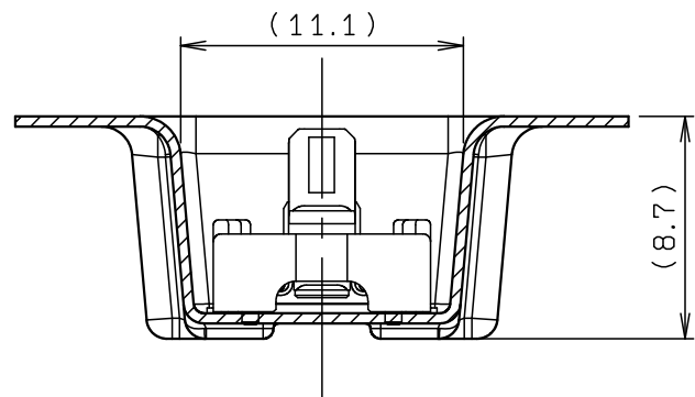
SECT. F-F (S=3:1)
