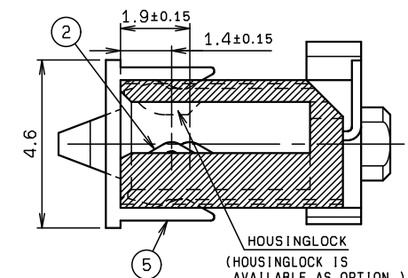
SECT. Y-Y (S=15:2)
