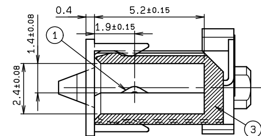
SECT. X-X (S=15:2)
