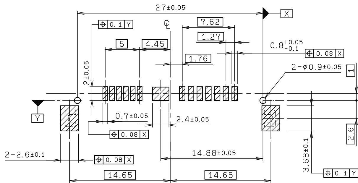
RECOMMENDED PCB LAYOUT FOR STD ANCHOR
