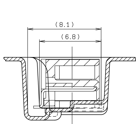
SECT. E-E
