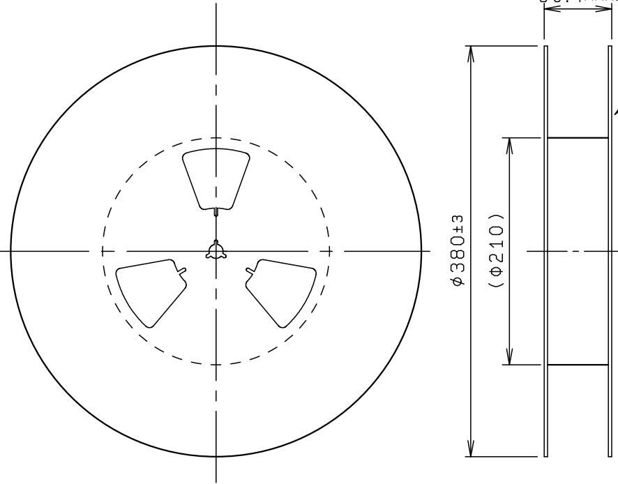
REEL DIMENSION (S=1:5)
