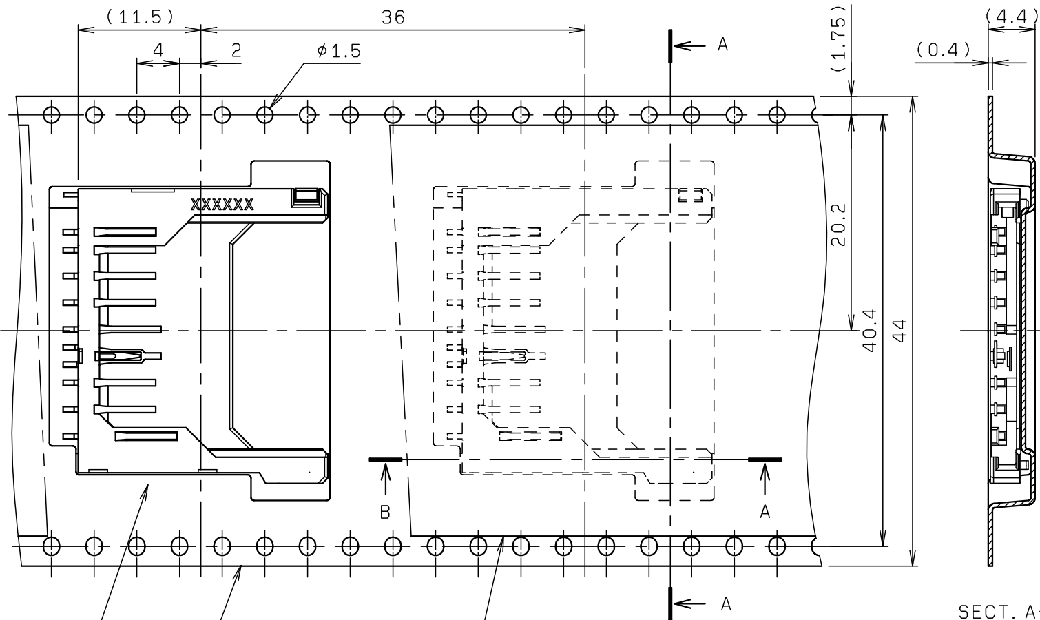
SECT. A-A
