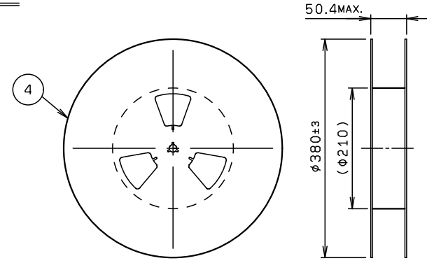
REEL DIMENSION
