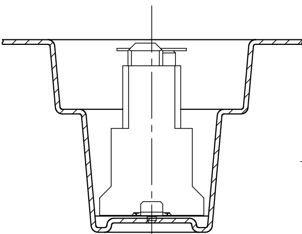
SECT. N-N (S=3:1)
