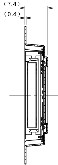
SECT. D-D
