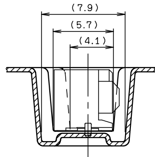
SECT. E-E (S=4:1)
