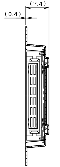
SECT. F-F
