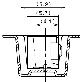
SECT. E-E (S=4:1)
