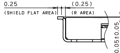
DETAIL "A" (S=10:1)
