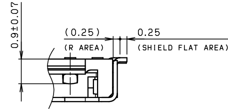
DETAIL "B" (S=10:1)
