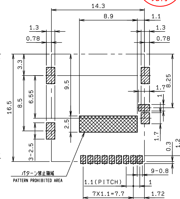
RECOMMENDED PCB PATTERN LAYOUT
