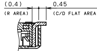
SECT. X-X (S=10:1)
