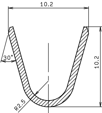
SECT. X-X
