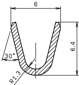
SECT. W-W
