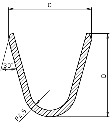
SECT. X-X
