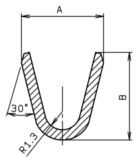
SECT. W-W
