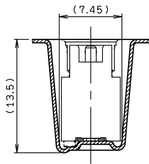
SECT. F-F (S=3:1)
