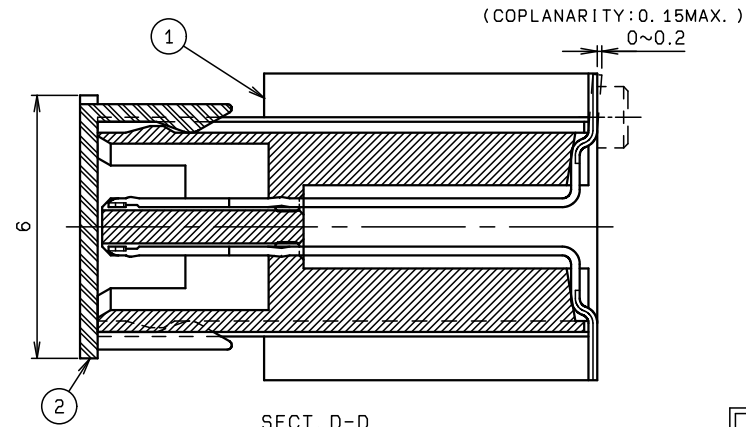
SECT. D-D
