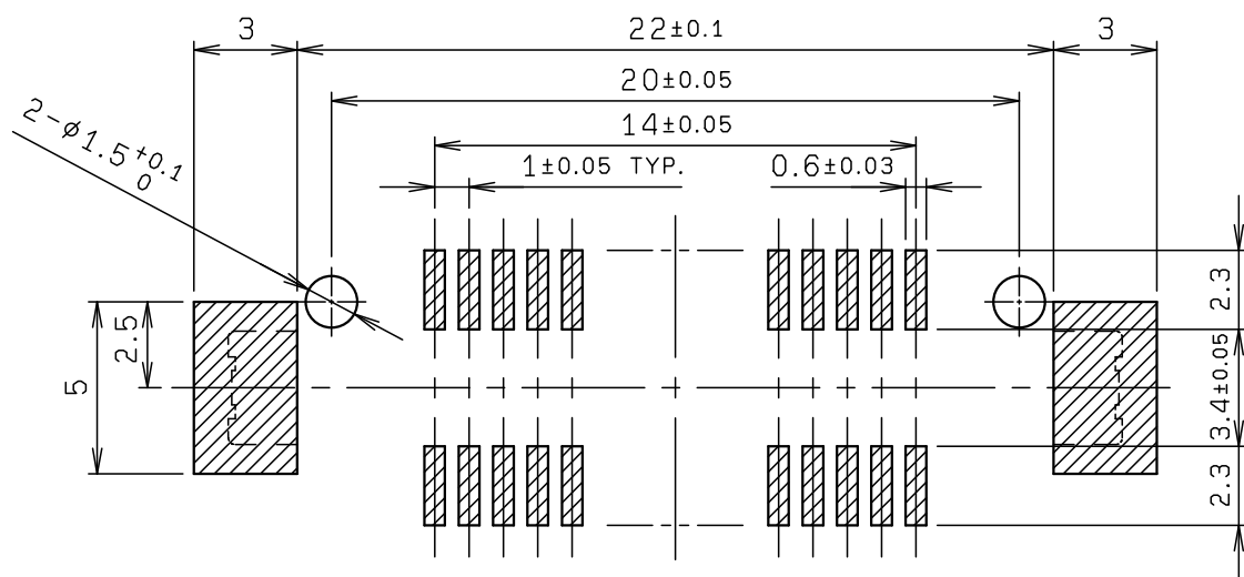
MOUNTING LAYOUT
