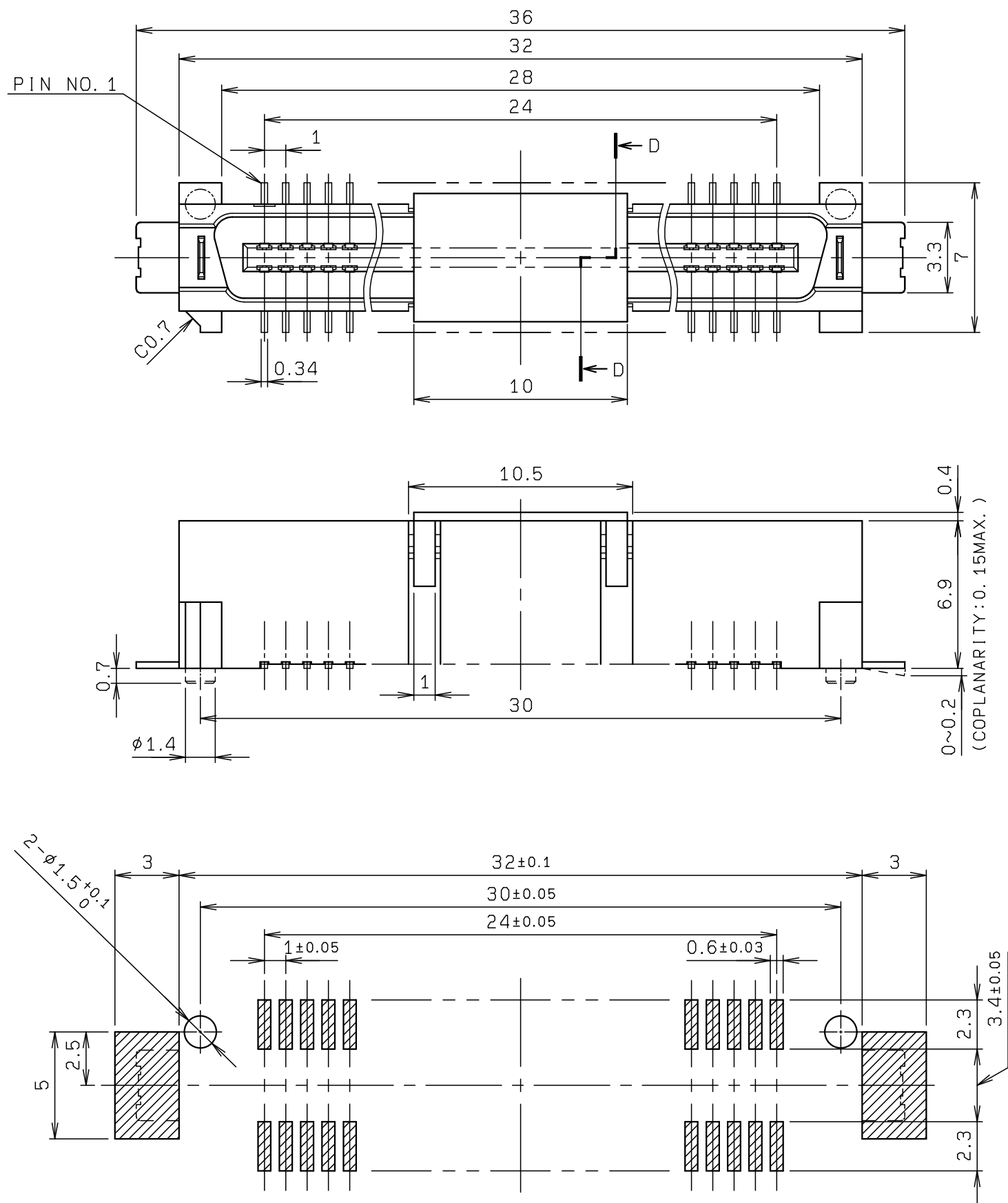
RECOMMENDED PATTERN
