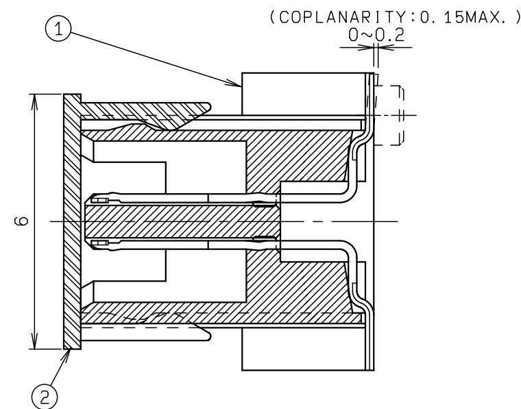
SECT. D-D
