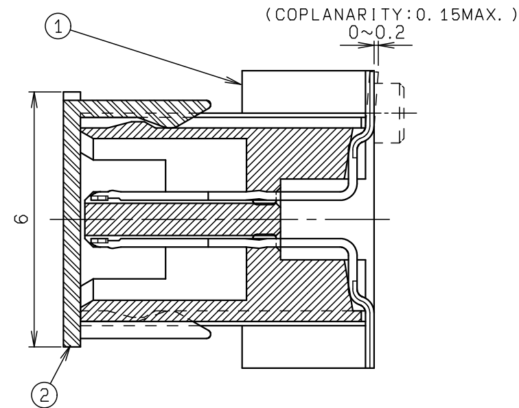
SECT. D-D
