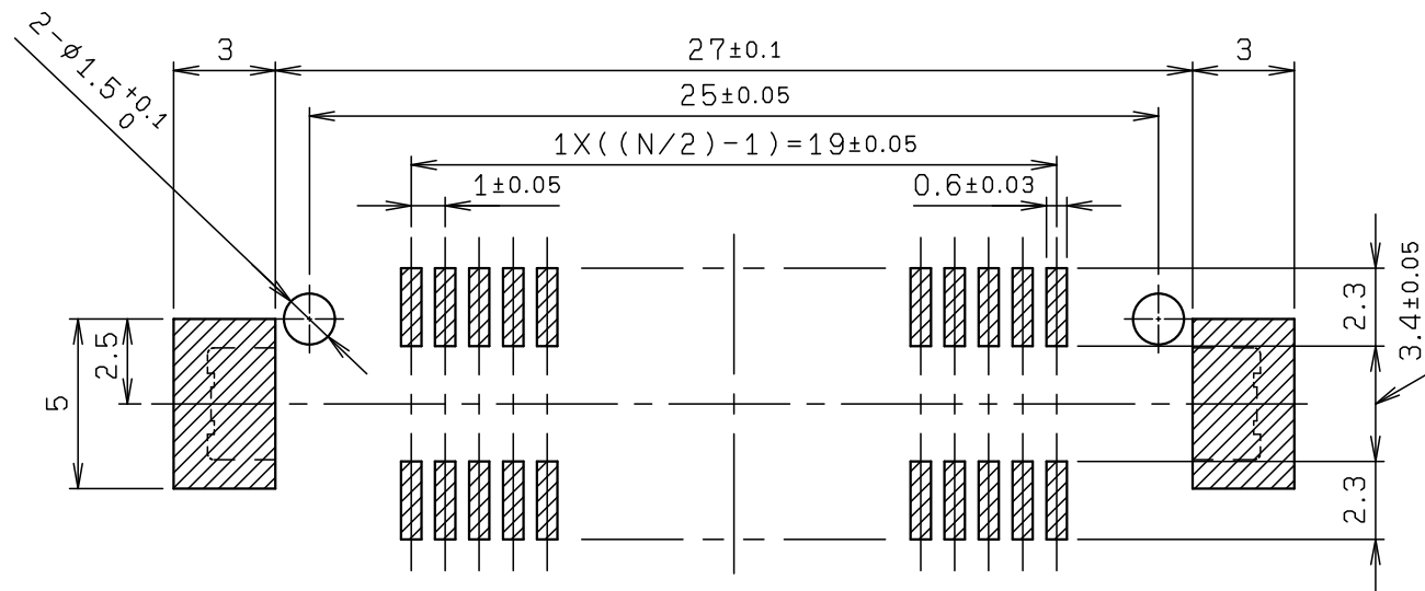
RECOMMENDED PATTERN
