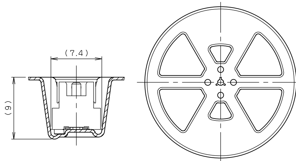
SECT. F-F (S=3/1)
