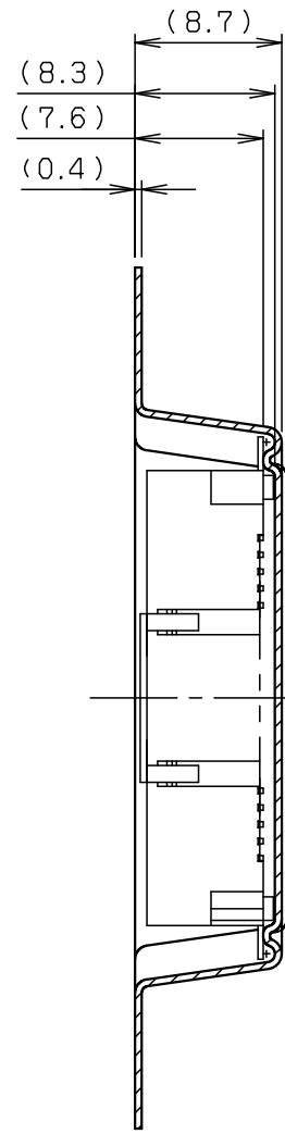
SECT. E-E
