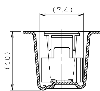
SECT. F-F
