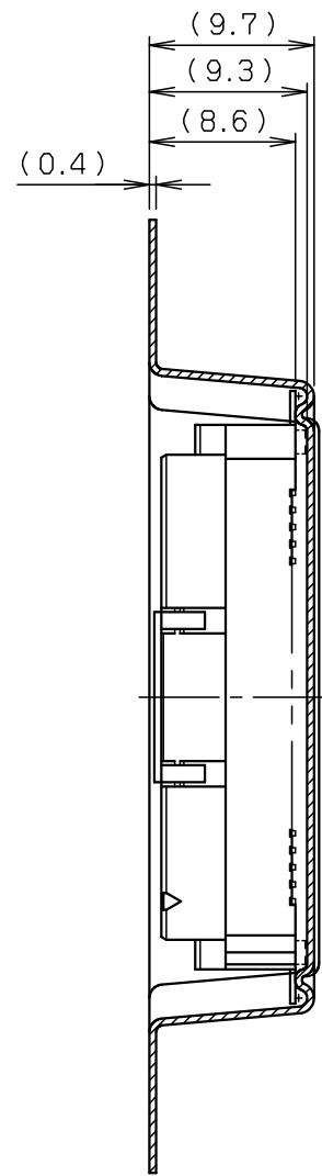
SECT. E-E
