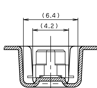
SECT. F-F (S=5:1)
