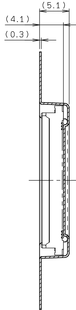
SECT. F-F
