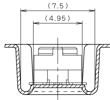
SECT. E-E (S=5:1)
