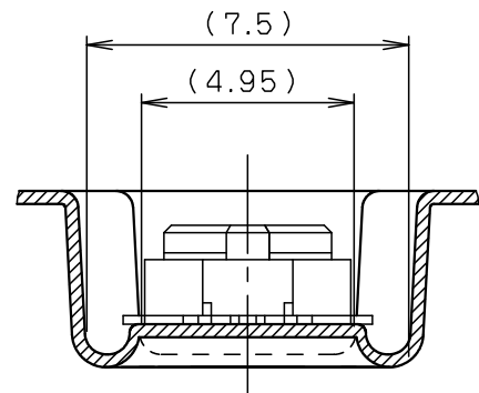
SECT. E-E (S=5:1)
