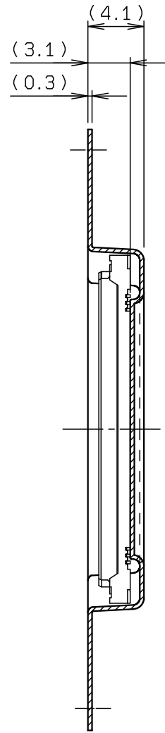
SECT. F-F
