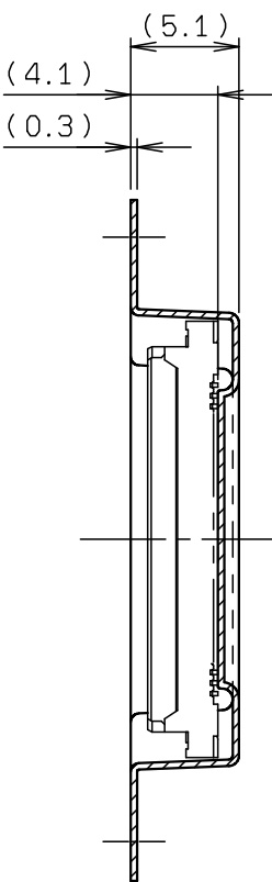
SECT. F-F
