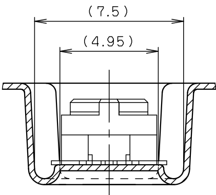
SECT. E-E (S=5:1)
