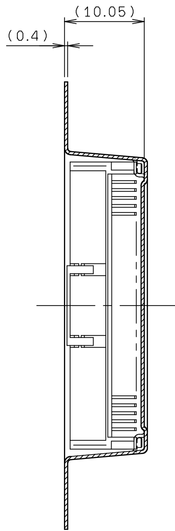
SECT. E-E
