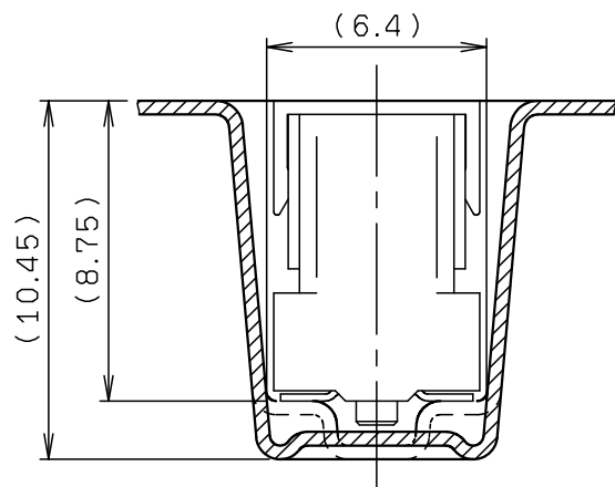
SECT. F-F (S=4:1)
