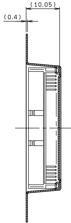
SECT. E-E
