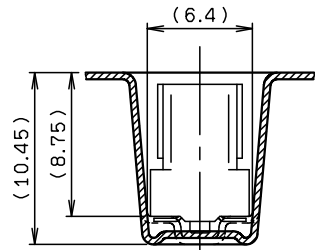
SECT. F-F (S=3:1)
